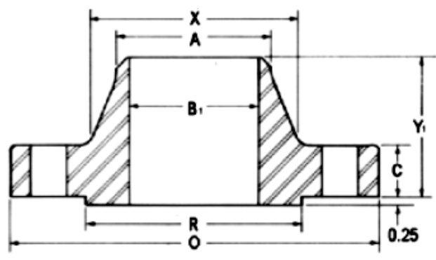
Weld Neck
